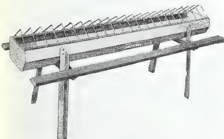
No. 255—5 feet long. Trough 9 inches wide, 4 1/2 inches deep, holds 40 pounds or 4 1/2 pecks dry laying mash. Serves 60 hens. Three in carton K.D. Weight 53 lbs. Second class freight L.C.L. Price: $6.00, not prepaid.
